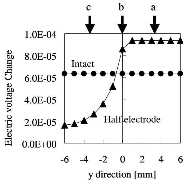
Fig. 8 Electric voltage change due to piezoresistivity
