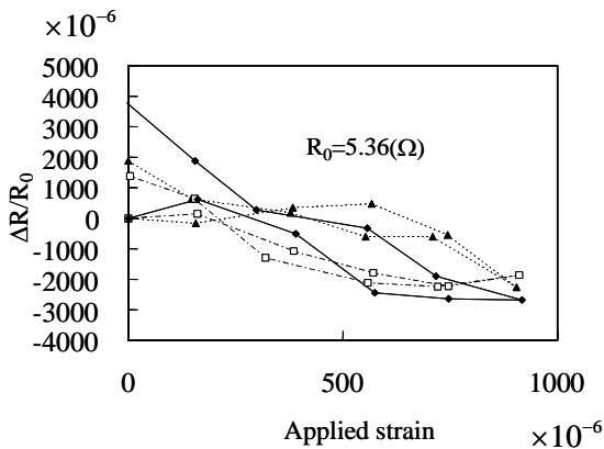
Fig.5 Measured piezoresistivity due to tensile strain (without polishing specimen surface)
