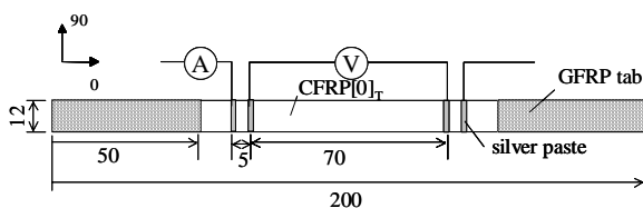
Fig. 1 Specimen configuration
