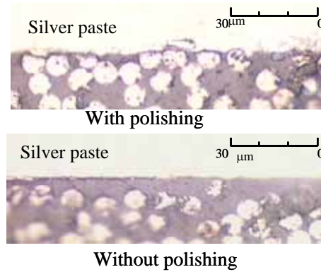
Fig.6 Cross section of the electrodes of both specimens.
