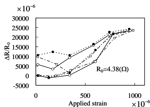
Fig.4 Measured piezoresistivity due to tensile strain (without polishing specimen surface)
