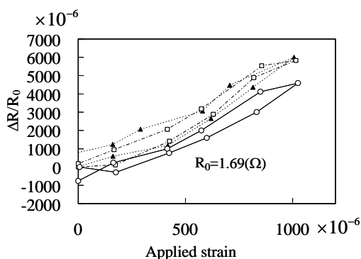
Fig.3 Measured piezoresistivity due to tensile strain (with polishing specimen surface)
