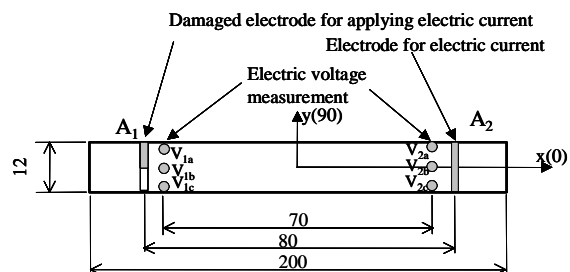
Fig.2 FEM model
